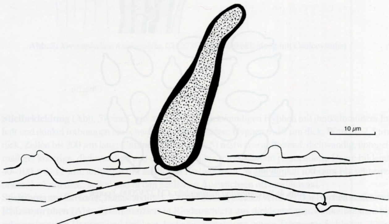
Abb. 2: Xeromphalina fraxinophila , CH 273/2000, Pileocystide
